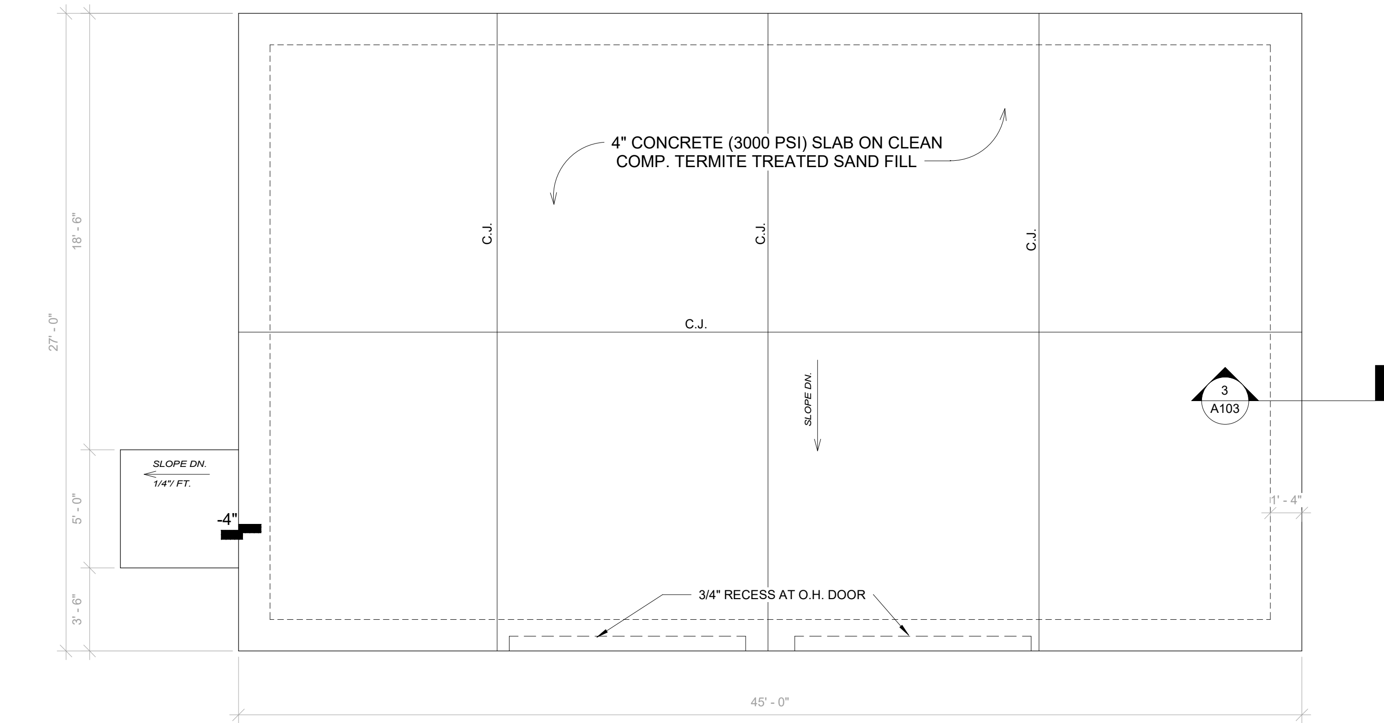
1 FOUNDATION PLAN 1/4" = 1'-0"
