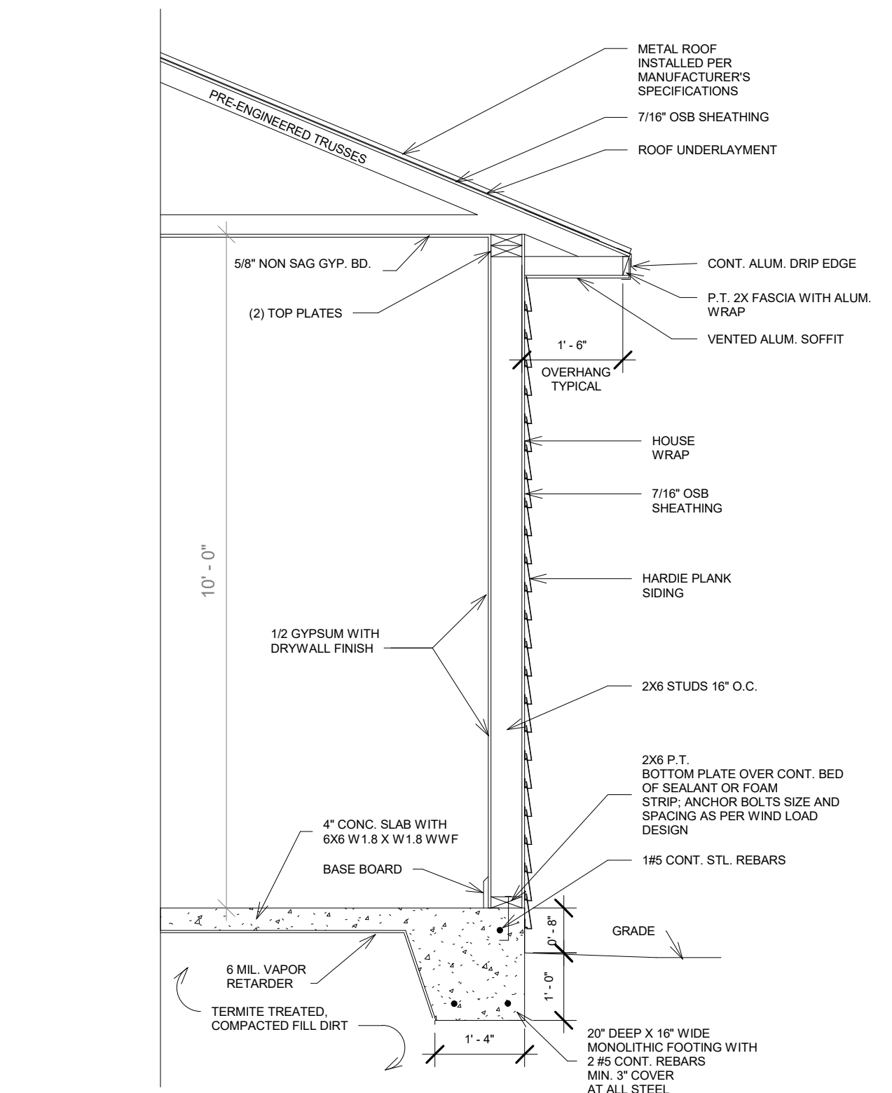
3 TYPICAL WALL SECTION 1/2" = 1'-0"
